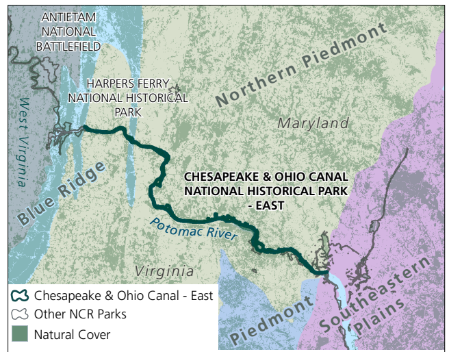
C&O CANAL - EAST IN CONTEXT. CHO-E passes primarily through the Northern Piedmont (beige), but also touches the Blue Ridge (blue) and Southeastern Plains (pink). Areas of natural vegetation cover are represented by darker shading on the map.
