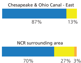
Observed Climate Change Vulnerability (1981 – 2014)
