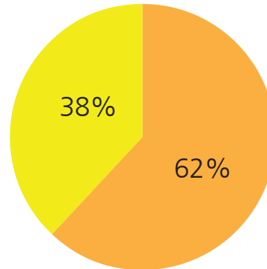
Near Future Climate Change Vulnerability CHOH-E (through 2040)
