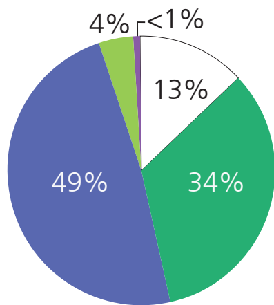
Observed Climate Change Vulnerability CHOH-E (1981 – 2014)
