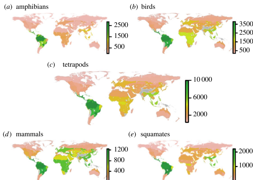
Figure 2. Global species richness maps. Species richness was computed by bioregion for tetrapods (c), amphibians (a), birds (b), mammals (d) and squamate reptiles (e).
